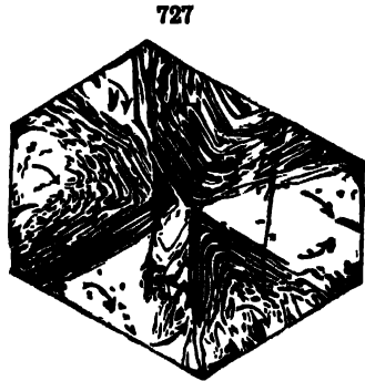
Basal section in polarized light, showing interpenetration of right- and left-handed portions. Des Cloiseaux.
